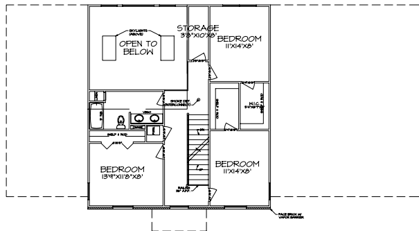
SECOND FLOOR PLAN A-3 SCALE: 1/4"=1'-0"
