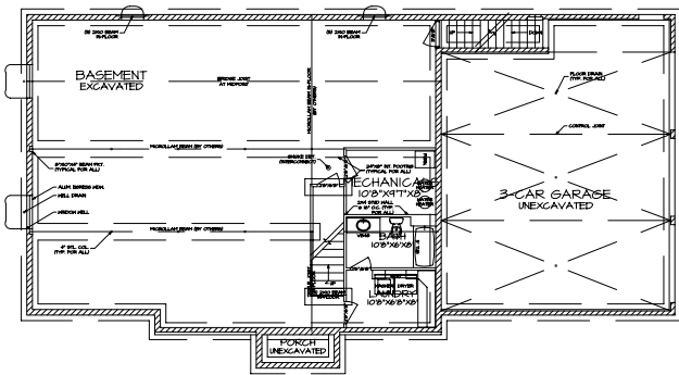
FOUNDATION PLAN A-2 SCALE: 1/4"=1'-0"
