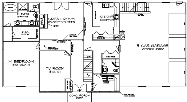
FIRST FLOOR PLAN A-2 SCALE: 1/4"=1'-0"
